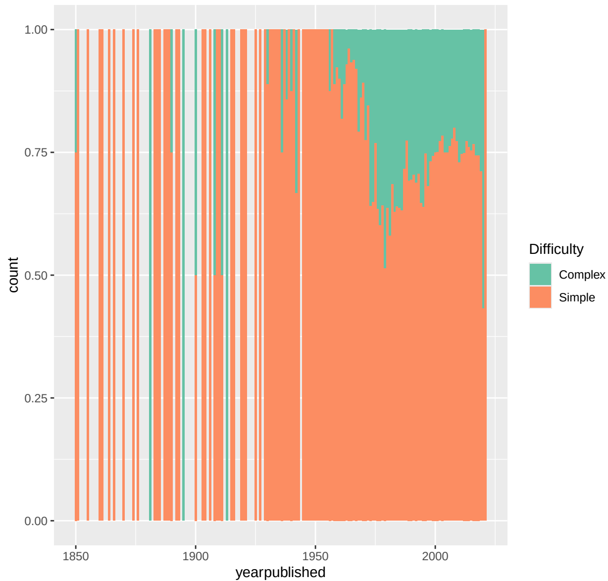
Difficulty Proportions Over Years
